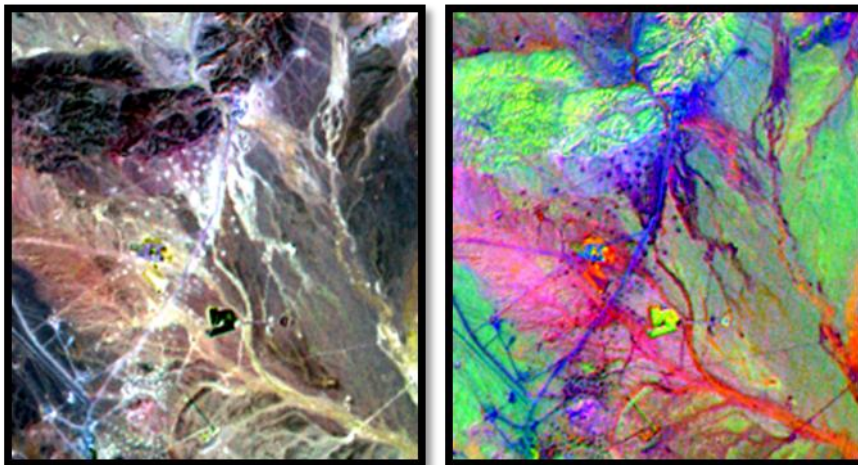
Fig. 2 (a) Image created by the PCA method; (b) image created by the use of bands 24, 53, 143.
