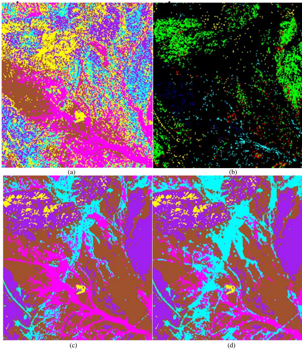
Fig. 3 Comparison of the classification results (cyan-urban, dirt road, yellow-mine area, sienna-soil, magenta-bare soil, purple-bedrock). Classified images using (a), (b) spectral angle mapper classification, and (c), (d) maximum likelihood classification defined by spectral knowledge, PC bands.
