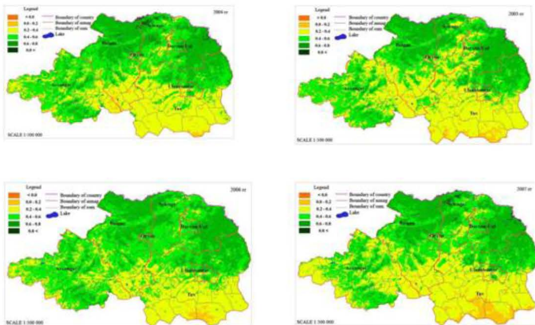
Figure 2: Distribution of the average vegetation index NDVI by years for the Northern part of Central Mongolia (May - September 2000 – 2010, comments in the text)
