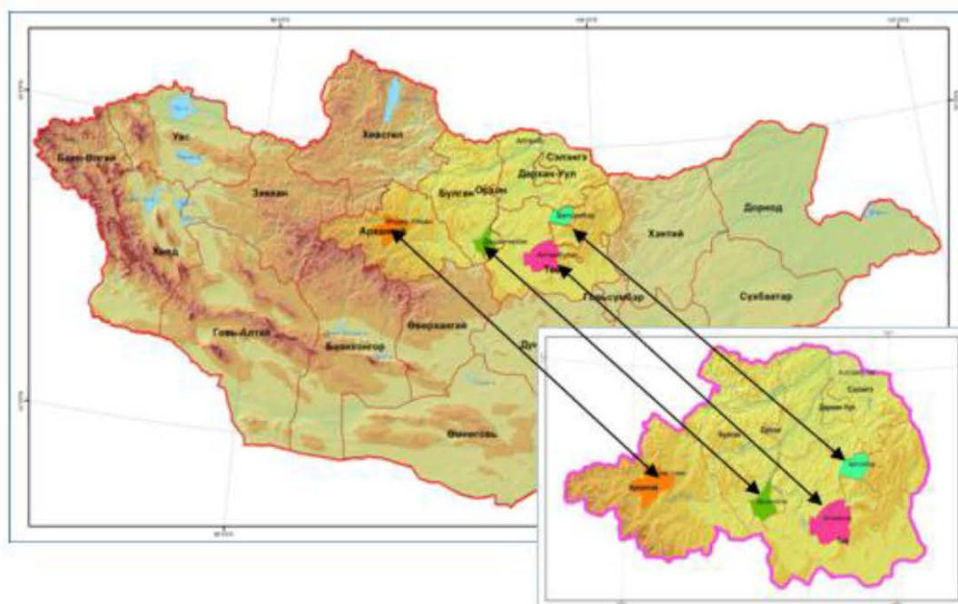
Figure 1: Location of the area being investigated on the map of Mongolia
